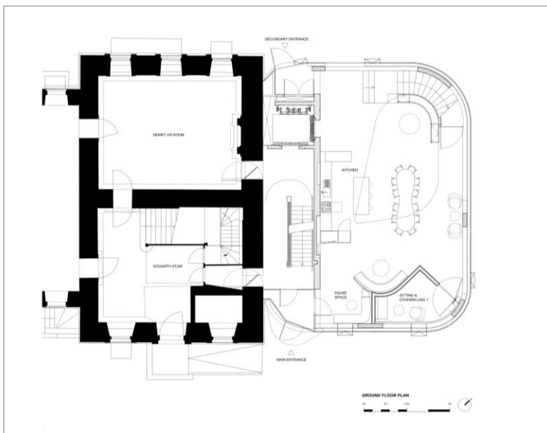
Ground floor, © Courtesy of Steven Holl Architects
