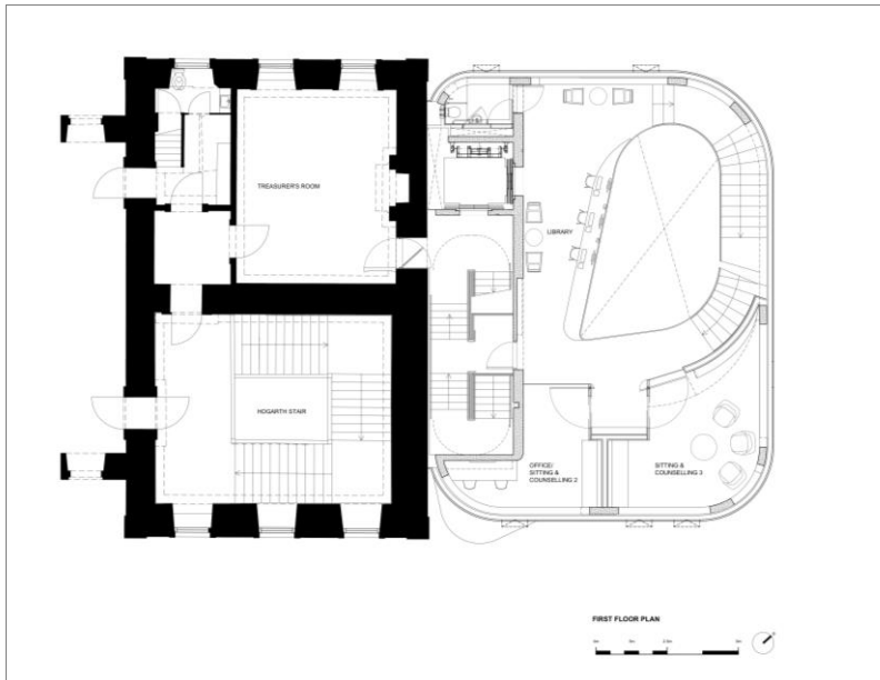
1 st floor, © Courtesy of Steven Holl Architects
