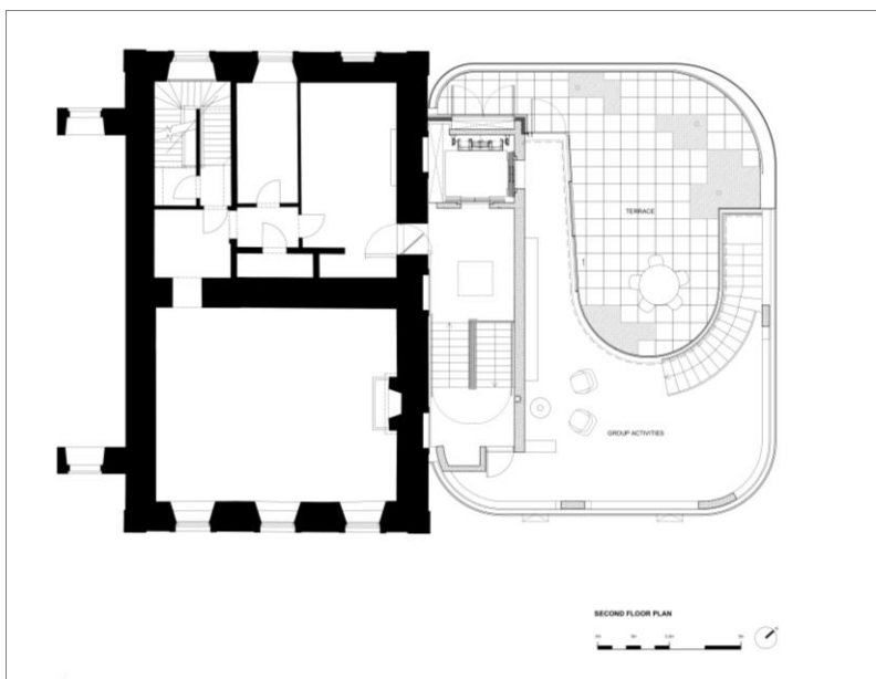
2 nd floor, © Courtesy of Steven Holl Architects
